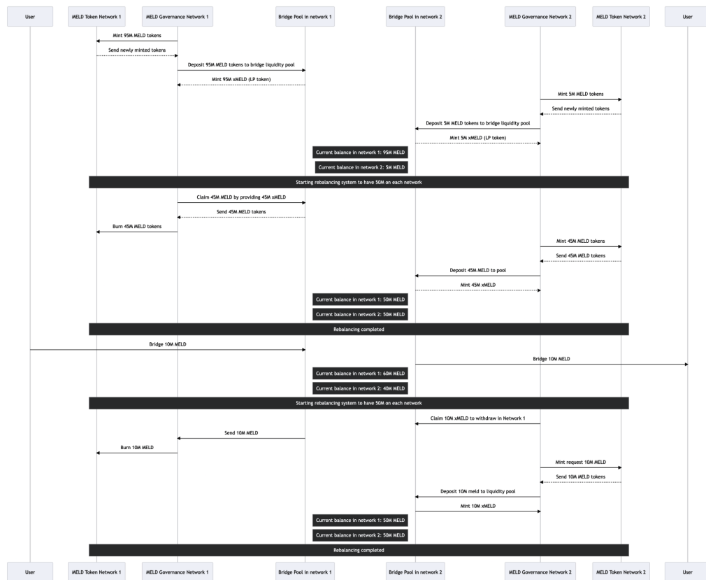
(Fig 20. sMELD multi-chain token rebalancing graph)
